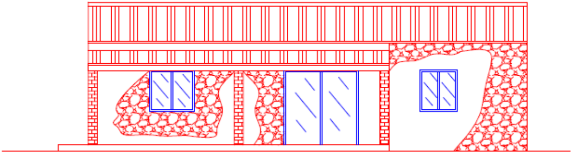
ALZADO PRINCIPAL
